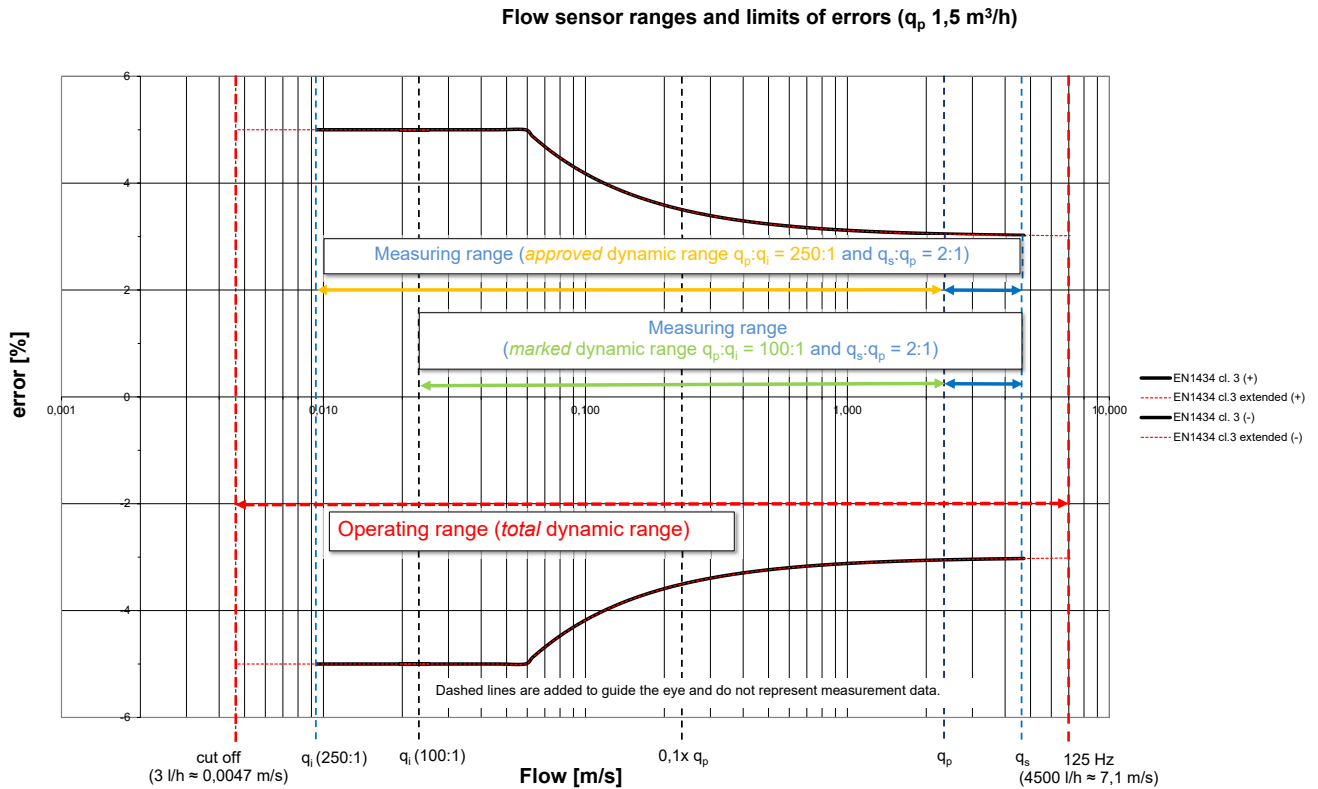
Figure 1: Operating (total dynamic) range and measuring (dynamic) range of a flow sensor with q_p 1,5 m 3 /h.
