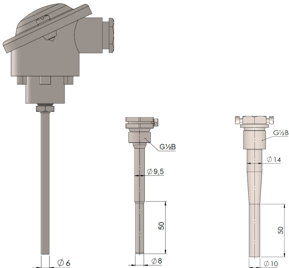
Figure 12: \varnothing 6,0 mm pocket sensor with connection head and corresponding pockets.
