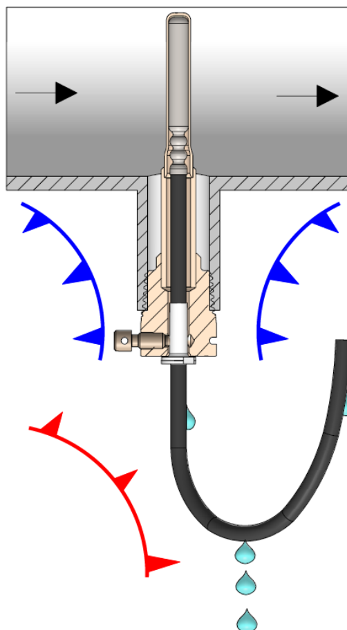
Figure 35: Correct installation of a temperature sensor for use in cooling measurements by which gravity prevents the penetration of condensation.
