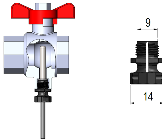
Figure 10: \varnothing 5,2 mm temperature sensor with composite union mounted in a ball valve.
