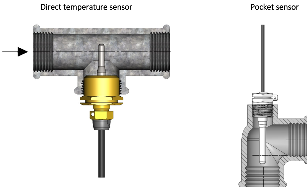
Figure 7: Illustration of a direct temperature sensor and a pocket sensor.
