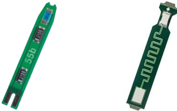
Figure 5: Thin film resistors mounted on a printed circuit board (PCB) [3,4].
