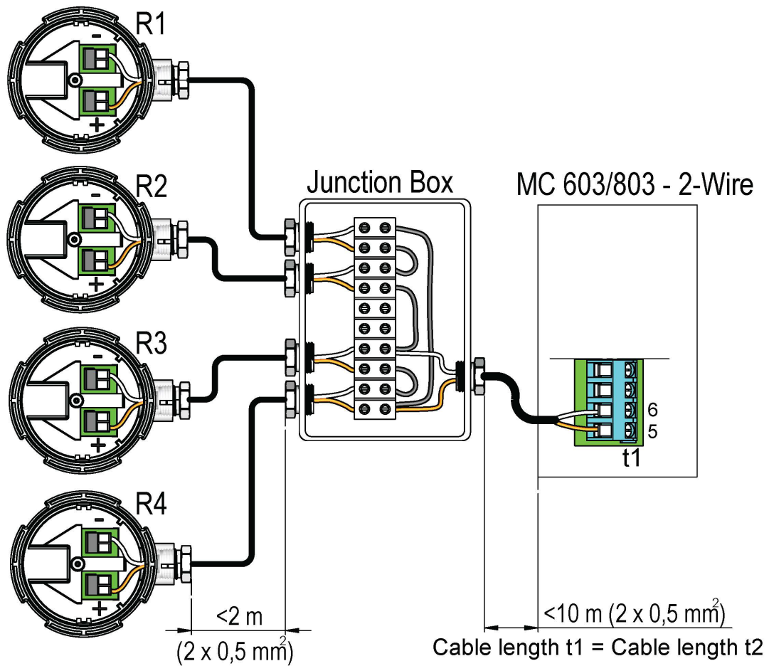
Figure 25: Example of an installation of 4 temperature sensors in one pipe. The installation is carried out with 2-wire connection, which gives a limitation of the cable length of 10 m. In this example, the connection of t1 (inlet sensor) connected to the MULTICAL® 603 calculator is shown. The corresponding installation must be carried out for t2 (outlet sensor).
