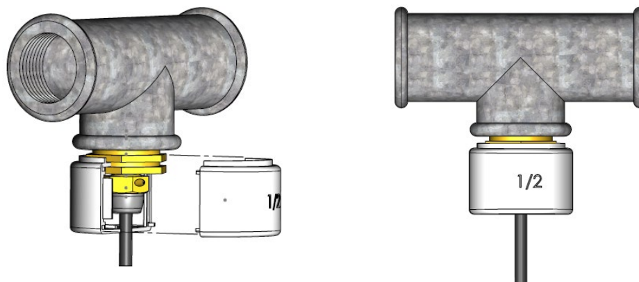
Figure 28: Examples of sealing of temperature sensors, either with sealing wire or sealing shells.
