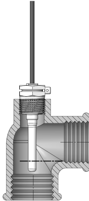
Figure 23: Example of correct installation of pocket sensor in a 90° angle.
