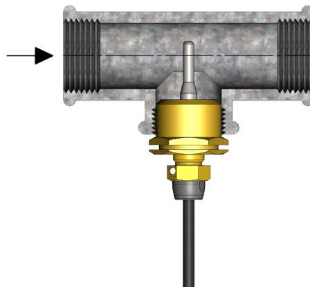
Figure 22: Example of correct installation of a direct short temperature sensor.
