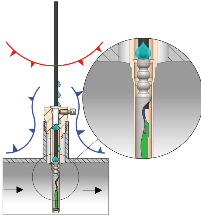
Figure 34: Penetration of condensation into a pocket sensor.
