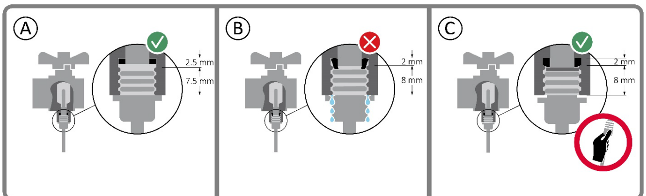
Figure 30: TemperaturSensor 63 \varnothing 5,0 or \varnothing 5,2 installed in ball valves (A) according to EN 1434:2022 or (B), (C) according to earlier versions of EN 1434
