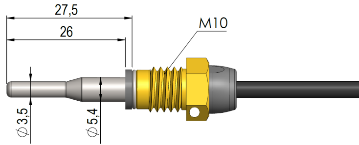
Figure 8: Direct short DS 27,5 mm temperature sensor.
