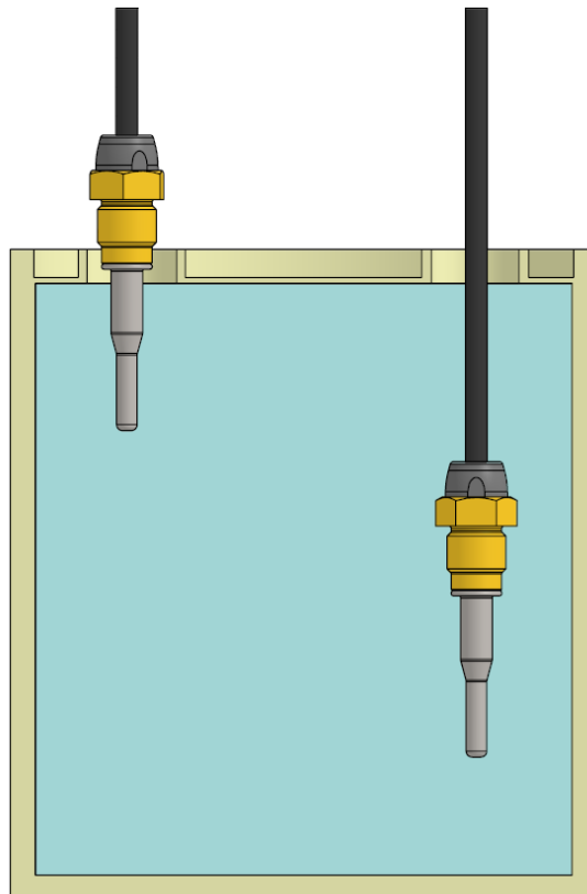
Figure 16: The qualifying immersion depth is determined by comparing the measurements of two temperature sensors that are fully and partially immersed in water, respectively.
