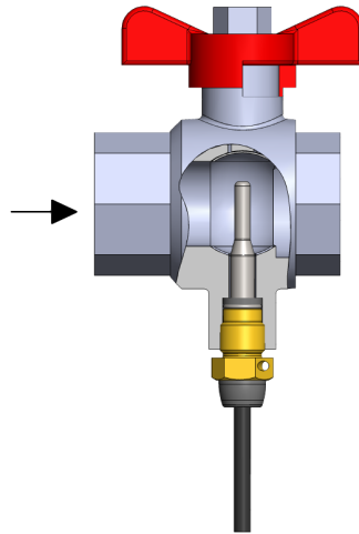
Figure 29: Direct short DS 27,5 mm temperature sensor mounted in a ball valve.
