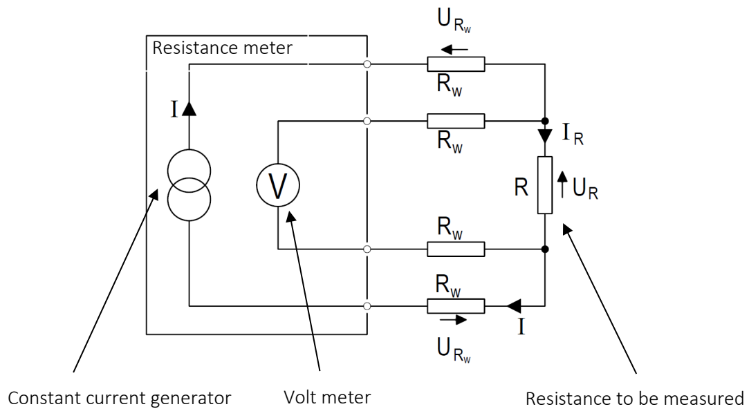
Figure 4: Measurement of resistance value by means of the 4-wire principle by which the wires do not influence the resistance measurement.
