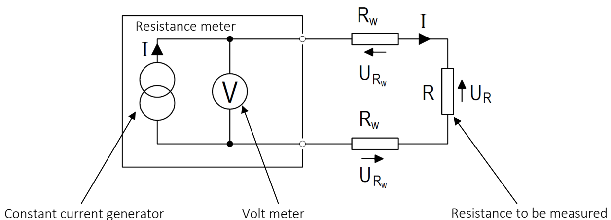
Figure 3: The influence of the wires on the measured resistance value.
