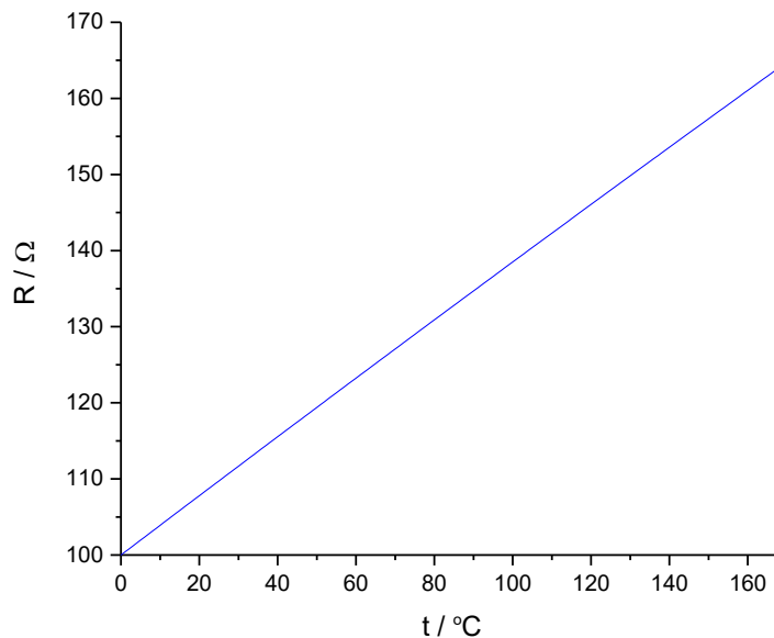
Figure 1: The correlation between the temperature, t , and the resistance, R , for a platinum Pt100 resistance temperature sensor with a resistance of 100\ \Omega at 0\ ^\circ\text{C} .
