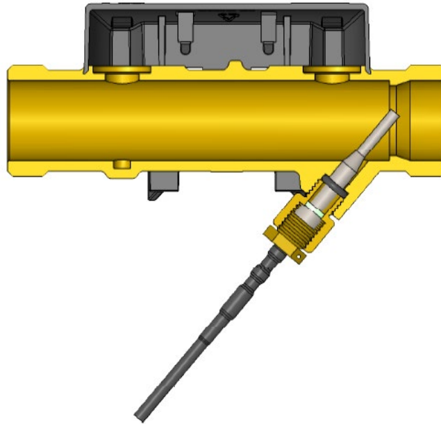
Figure 33: Direct short DS 38 mm temperature sensor mounted with 11 mm adapter in a flow sensor.
