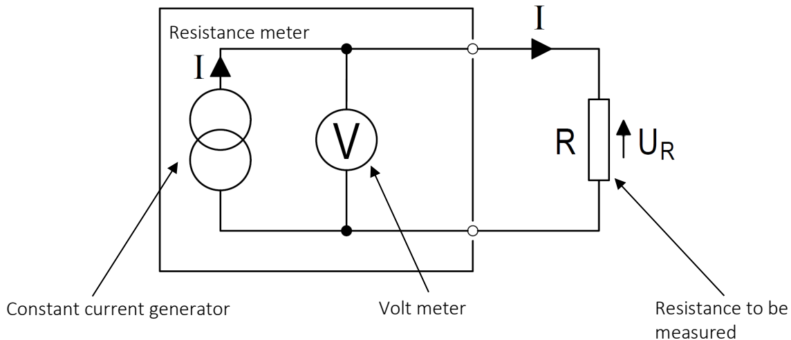
Figure 2: Measurement of a resistance value by means of a constant current ger
