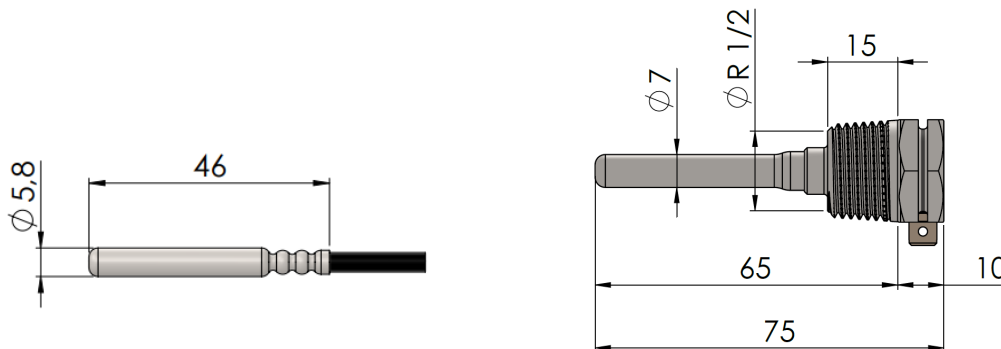
Figure 9: \phi 5,8 mm pocket sensor with corresponding 65 mm pocket.
