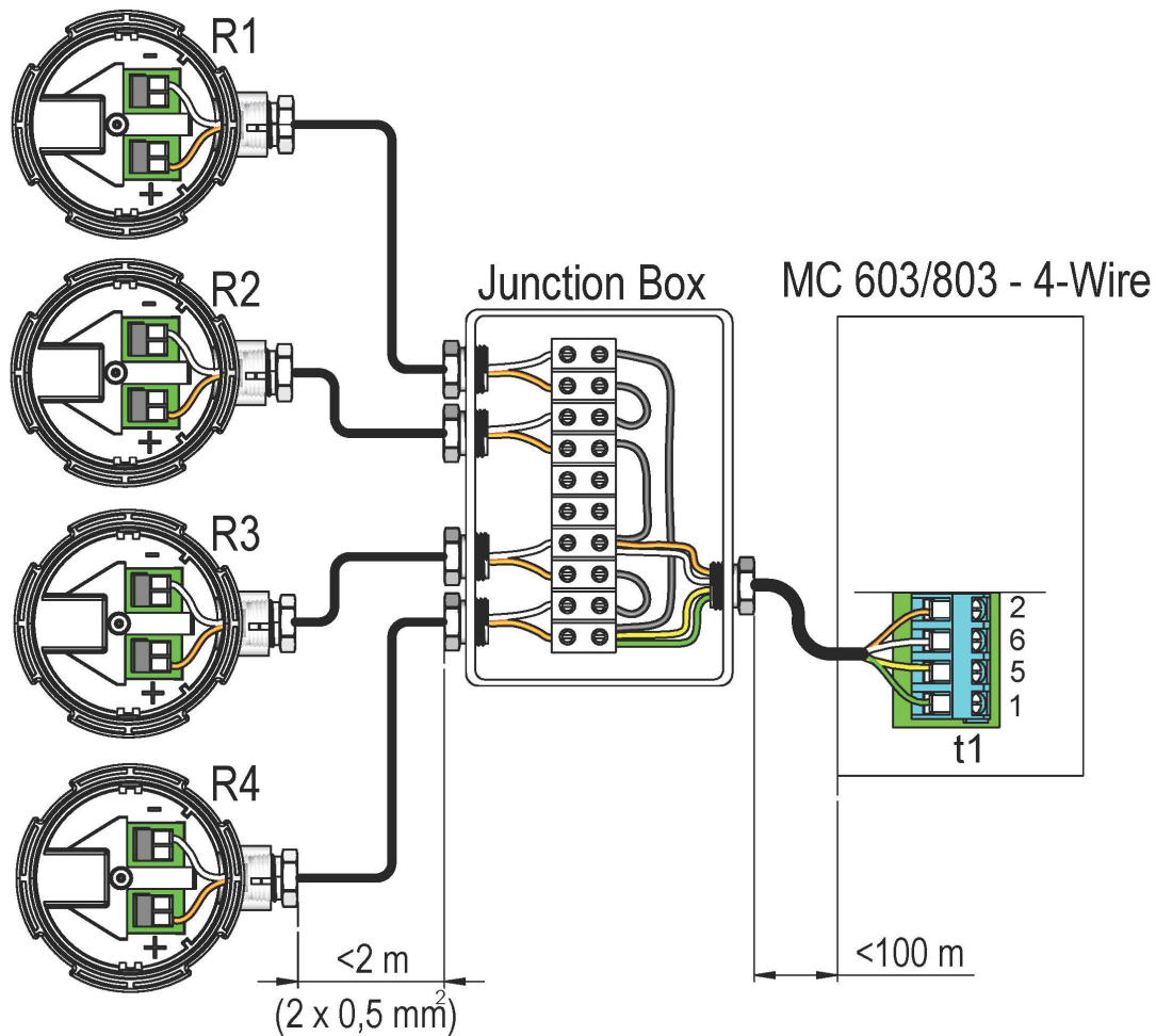
Figure 26: Example of an installation of 4 temperature sensors in one pipe. The installation is carried out with 2-wire connection in combination with 4-wire connection, which enables a cable length of up to 100 m between calculator and temperature sensors. In this example, the connection of t1 (inlet sensor) connected to the MULTICAL® 603 calculator is shown. The corresponding installation must be carried out for t2 (outlet sensor). Other approved calculators such as MULTICAL® 803 can be used in the same way.
