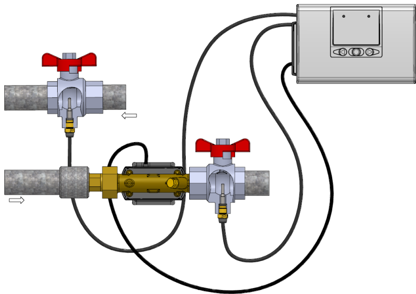
Figure 19: A typical heat or cooling meter installation in which one temperature sensor is installed in the inlet flow and the other one is installed in the outlet flow.
