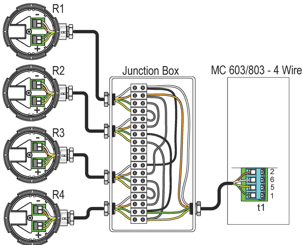
Figure 27: Example of an installation of 4 temperature sensors in one pipe. The installation is carried out with 4-wire connection, which enables a cable length of up to 100 m between calculator and temperature sensors. In this example, the connection of t1 (inlet sensor) connected to the MULTICAL® 603 calculator is shown. The corresponding installation must be carried out for t2 (outlet sensor). Other approved calculators such as MULTICAL® 803 can be used in the same way.
