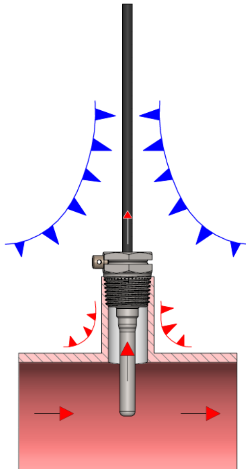
Figure 15: Illustration of heat conduction error in temperature measurement due to heat conduction into the surroundings.
