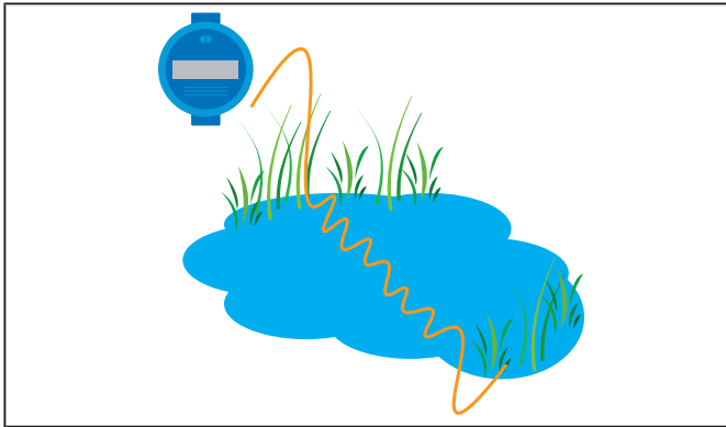
Example of the reflection on water.
