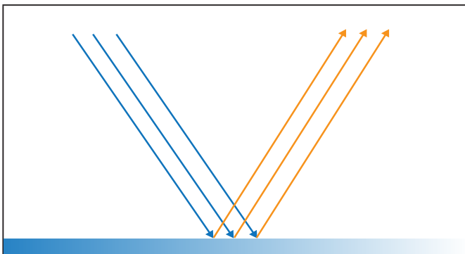
The reflection on a smooth surface.
