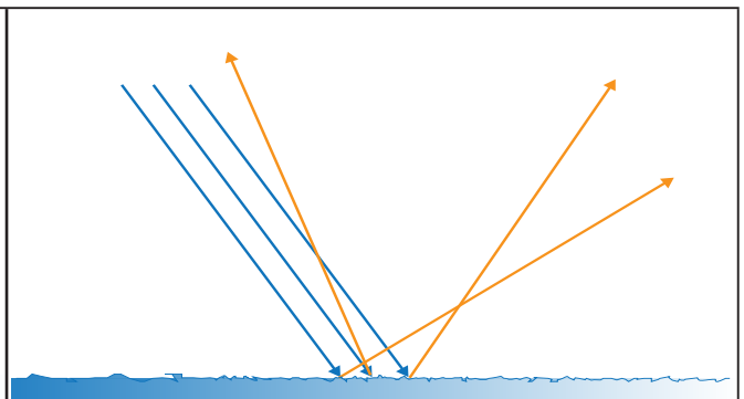
The reflection on an uneven surface.
