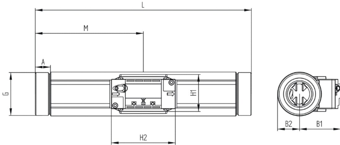
Figure 4: Flow sensor with G5/4 and G2 threaded connection
