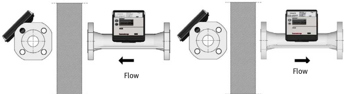
Figure 13: Flange meter
