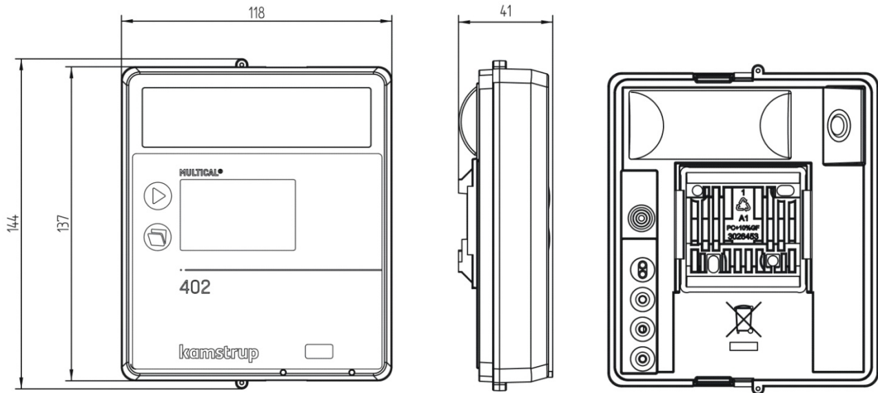
Figure 2: Mechanical dimensions of electronics unit
