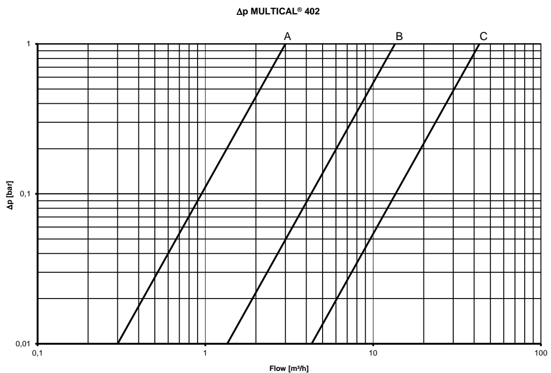
Diagram 2: Pressure loss graphs
