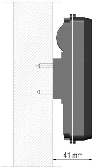
Figure 14: Wall mounted MULTICAL® 402
