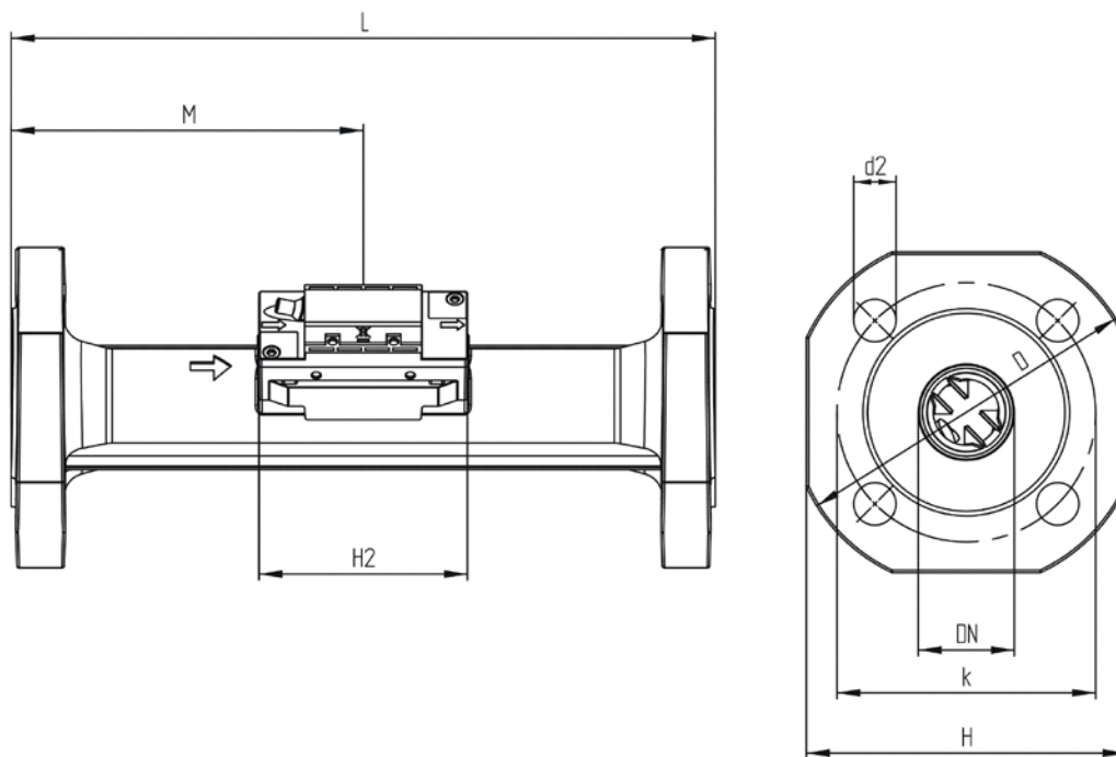
Figure 5: Flow sensor with DN25 to DN50 flange connection
