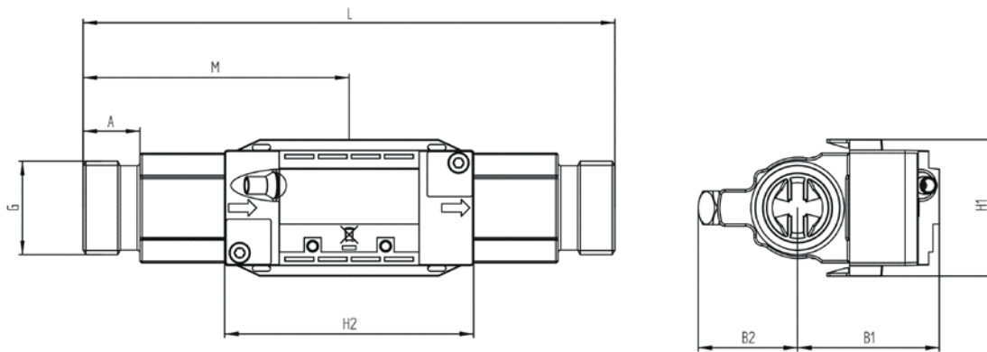
Figure 3: Flow sensor with G 3/4 and G1 thread connection
