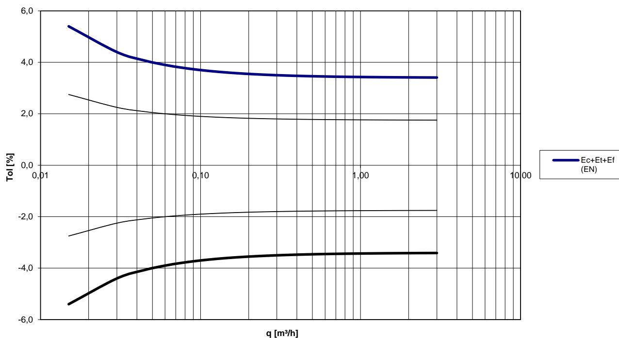
Diagram 1: Total typical accuracy of MULTICAL® 402 compared to EN 1434-1
