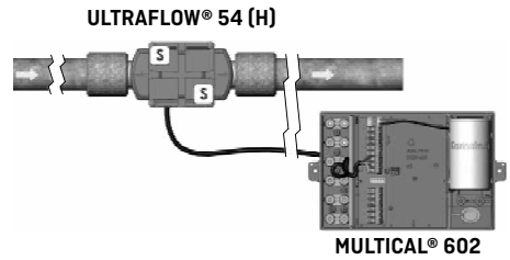
ULTRAFLOW® 54 DN150-DN250
