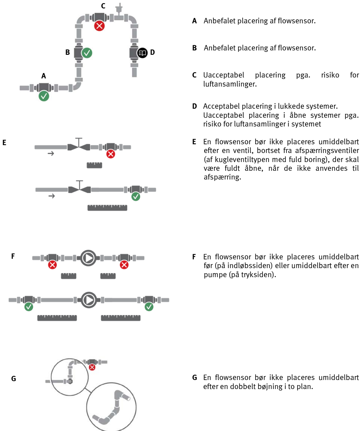
Figur 1. Generelle installationsanbefalinger for flowsensorer.
