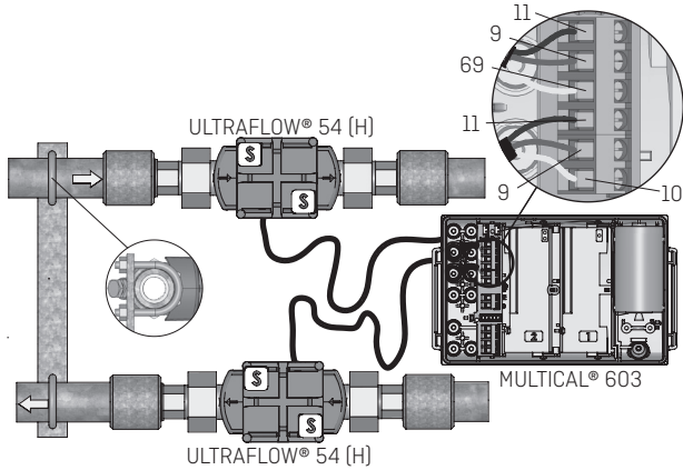
Figure 22. Direct electric connection of two ULTRAFLOW® flow sensors to MULTICAL® in an installation with equipotential connection [electric low impedance connection] between the pipes . No welded joints occur.
