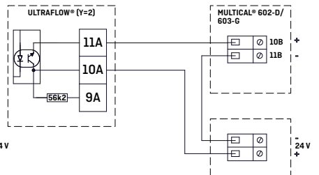
Figure 11. Two-wire connection of Pulse Transmitter/Pulse Divider with output module (Y=2) to MULTICAL® 603-G and external 24 VDC supply.
