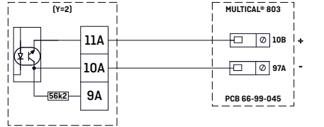
Figure 9. Two-wire connection of Pulse Transmitter/Pulse Divider with output module (Y=2) to MULTICAL® 803 with connection PCB for 24 V pulses.
