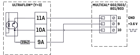
Figure 7. Three-wire connection of Pulse Transmitter/Pulse Divider with output module (Y=3) to MULTICAL® 602/603/801/803.
