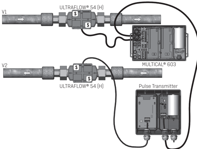
Figure 23. Installation of Pulse Transmitter for galvanic separation of one ULTRAFLOW® flow sensor [typically V2] in installations where an equipotential connection cannot be carried out. Electric welding can occur.
