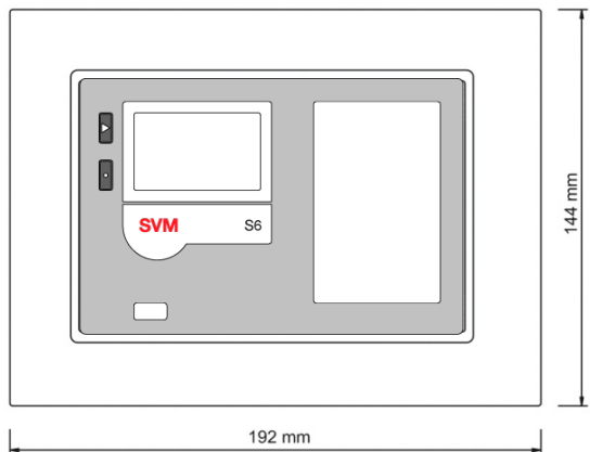
Panel-mounted SVM S6 seen from the front
