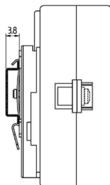
DIN rail mounting of MULTICAL® 602 is possible with a DIN rail bracket
