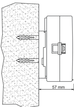
Wall-mounted SVM S6 seen from the side
