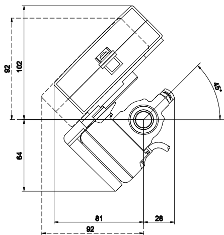
SVM S6 mounted on ULTRAFLOW®
