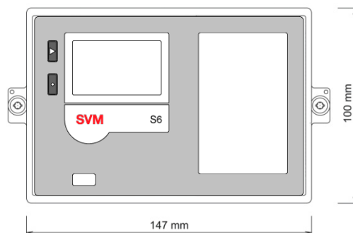
SVM S6 's front dimensions
