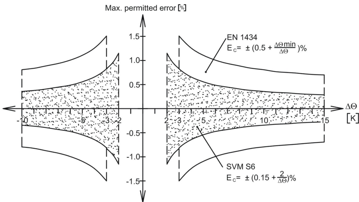
Figure 1. SVM S6 typical accuracy compared with EN 1434.
