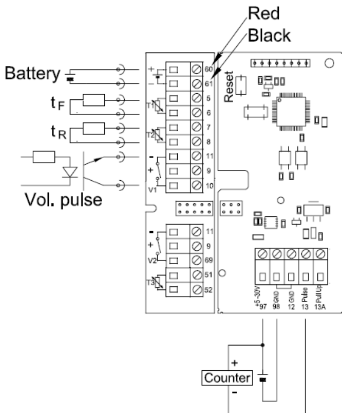
Verificationprint 5550-888 (to the right) with connection PCB 5550-492 (to the left)
