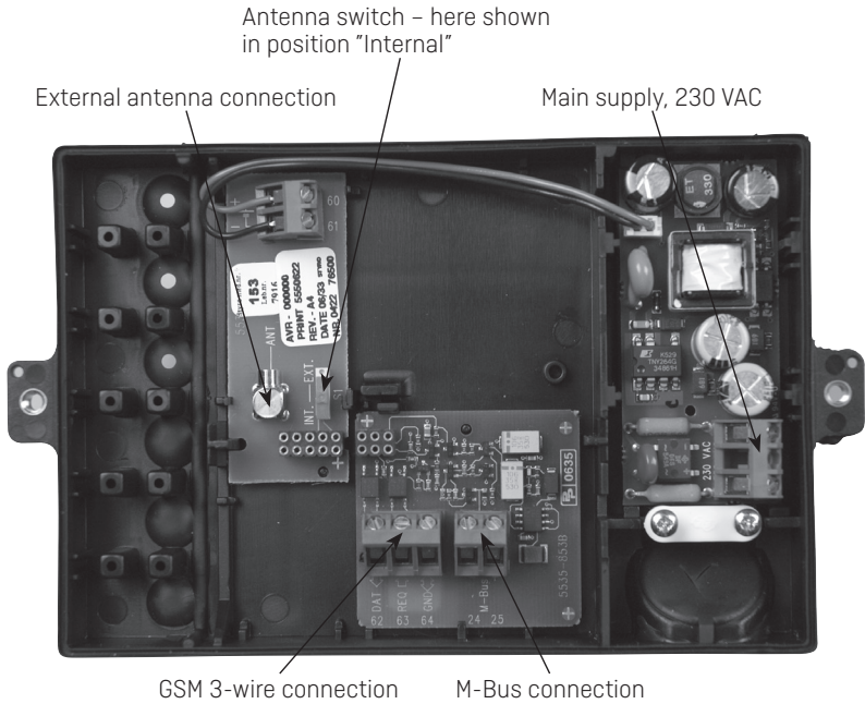
RF M-Bus Converter II, internal connections
