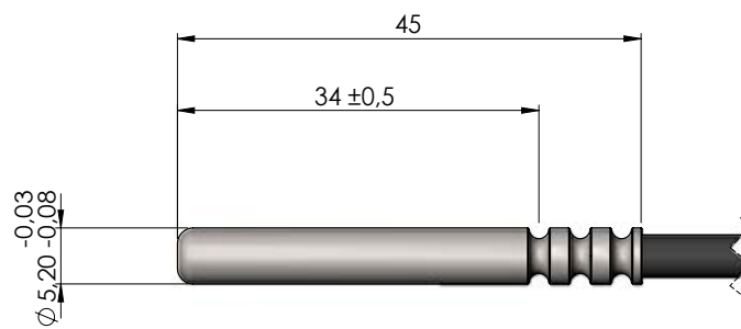
Temperature sensor
