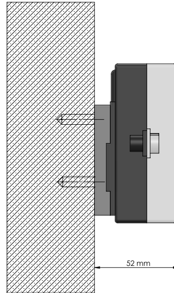
Wall-mounted MULTICAL® 602 seen from the side
