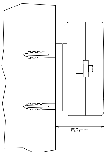
Wall-mounted MULTICAL® III from the side
