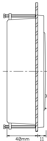
Panel-mounted MULTICAL® III, from the side
