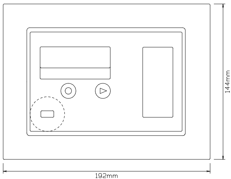
Panel-mounted MULTICAL® III, front view
