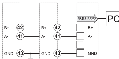
Fig. 25 Port RS485
