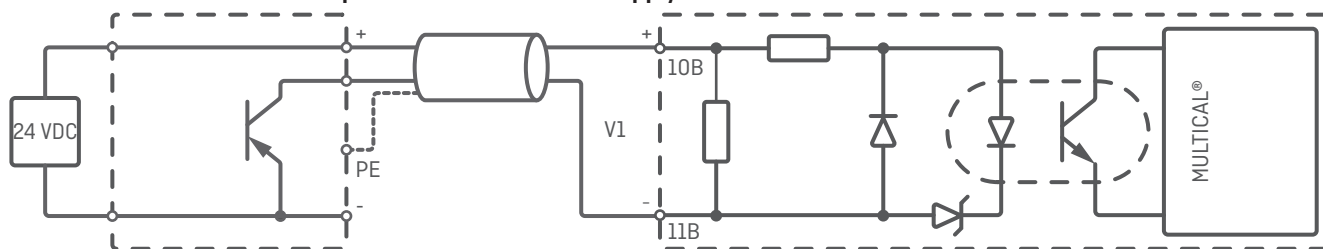
Flow sensor with transistor output and external 24 VDC supply
