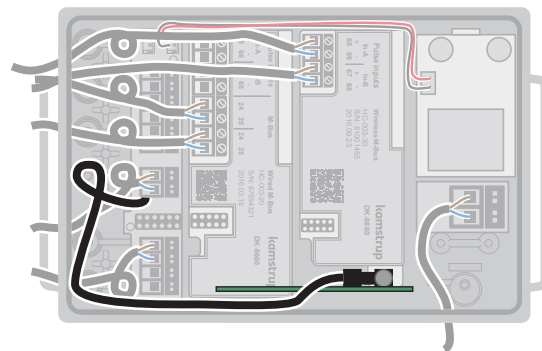
Wireless M-Bus-module with external antenna
