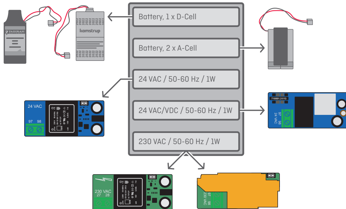
Figure 17: Choice of correct label for installed supply type
