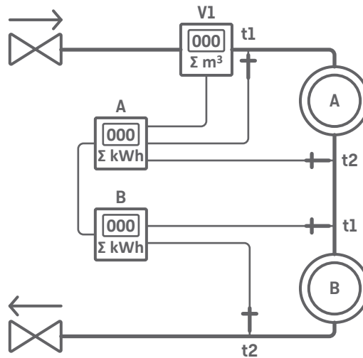
Figure 8: Heat installation with one flow sensor and 2 calculators.
