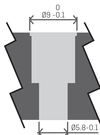
Figure 11: Measurement and tolerance requirements when installing a direct Ø5.0 mm or Ø5.2 mm temperature sensor.
