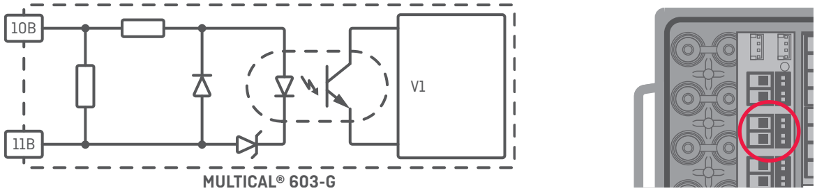
Figure 7: Opto-isolated pulse input (V1) on MULTICAL® 603-G (PCB 5550-1550).
