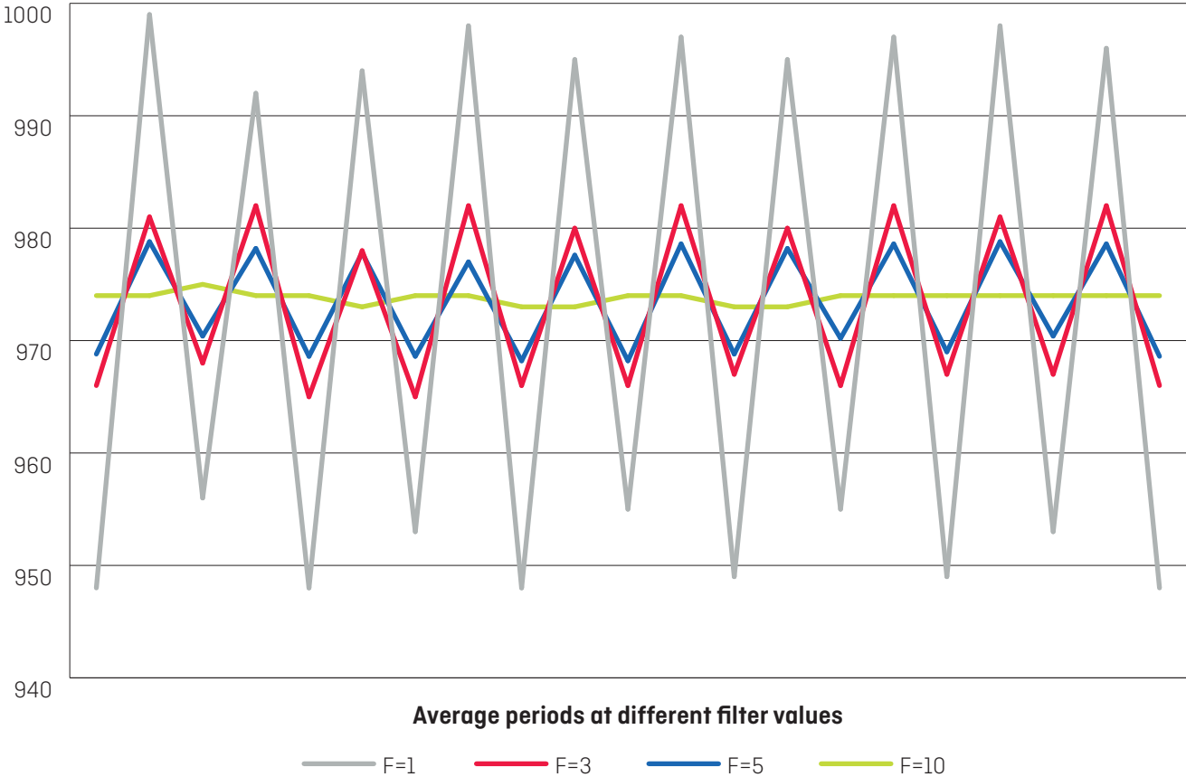
Actual flow rate at different filter values, F=1 to F=10
