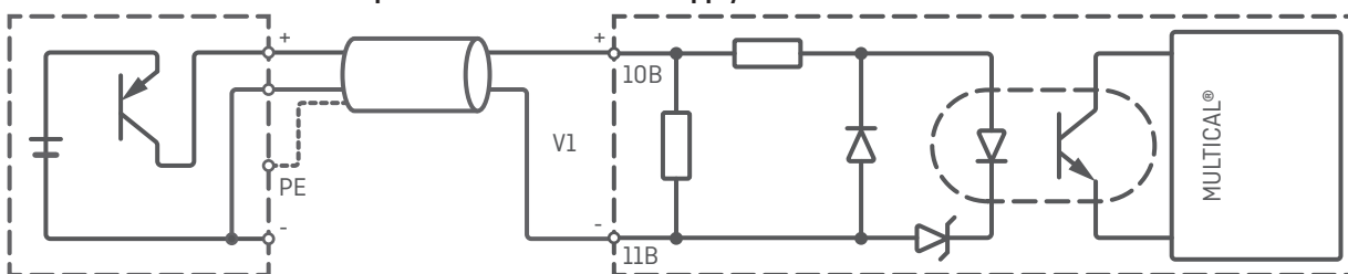
Flow sensor with transistor output and external 24 VDC supply
