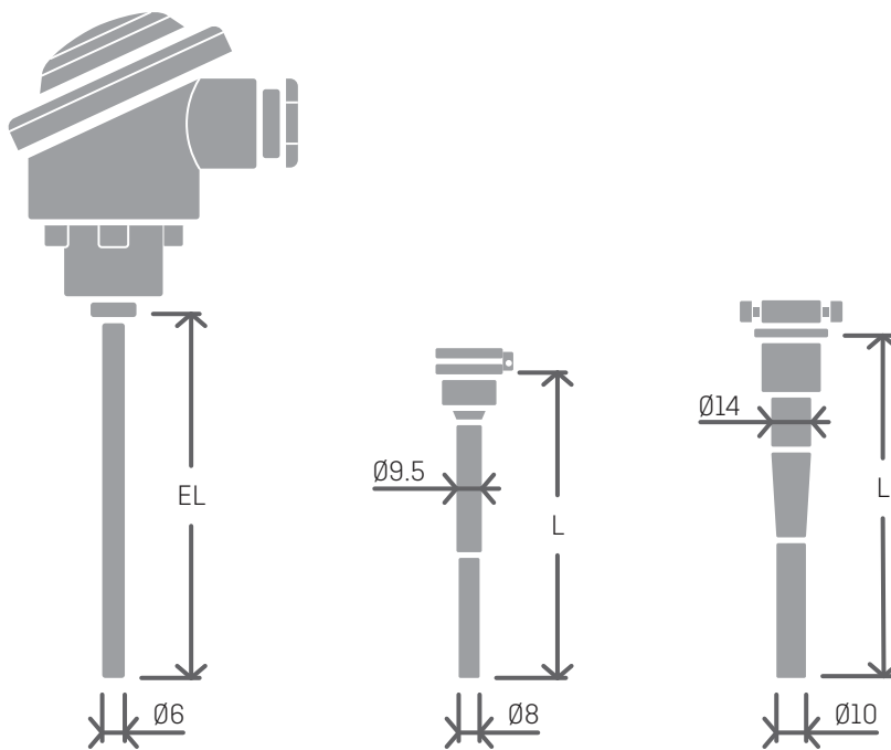
Figure 15: ø6 mm pocket sensor with connection head and matching pockets.
