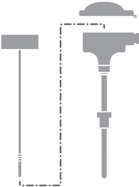
Figure 13: A \varnothing 5.8 mm pocket sensor with connection head can, for example, be mounted in a tee as shown in Figure 14
