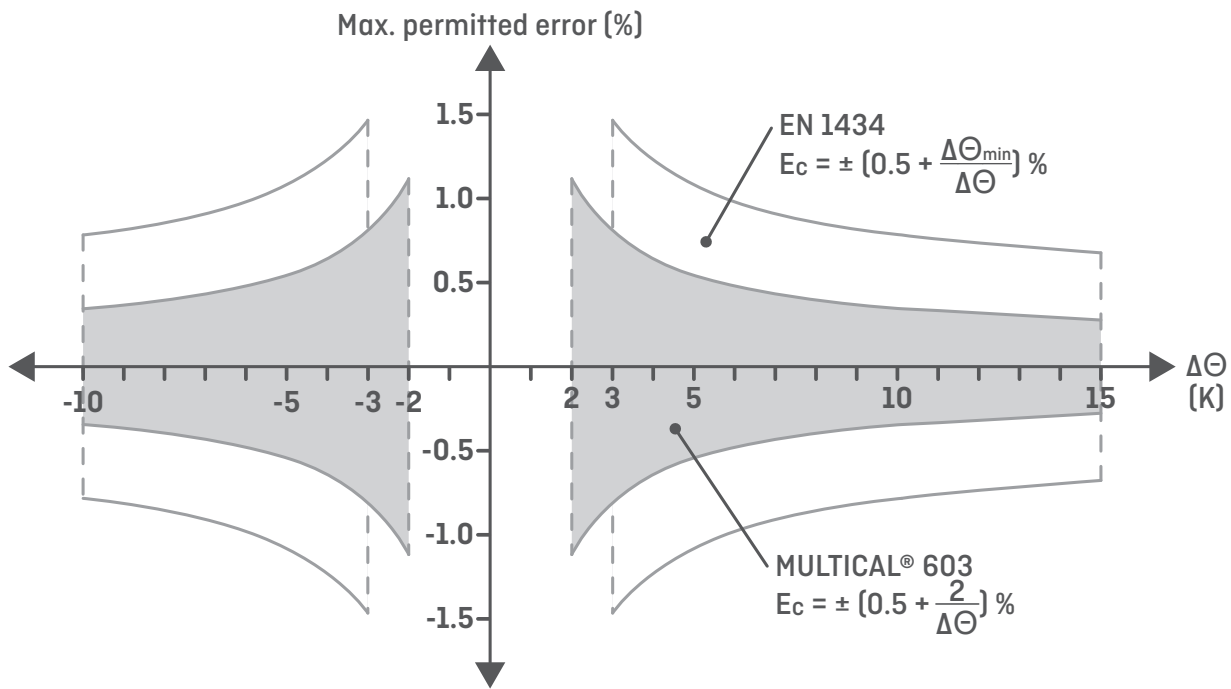
Figure 2: Typical accuracy of MULTICAL® 603 compared to EN 1434.
