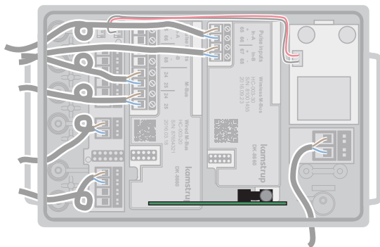
Wireless M-Bus-module with internal antenna
