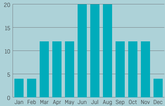
Scheduler function
