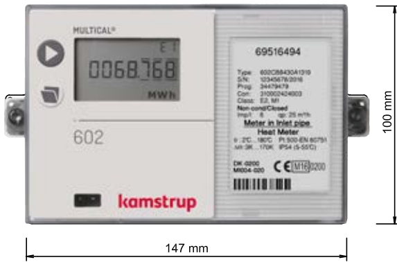
Panel mounted MULTICAL® 602 seen from the front
