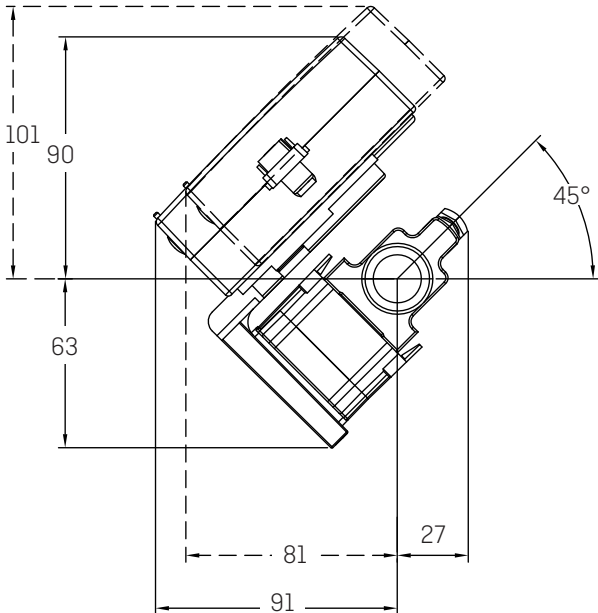
Front dimensions of MULTICAL® 602
