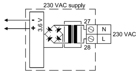
Figure 33. 230 VAC supply module for Pulse Transmitter/Pulse Divider
