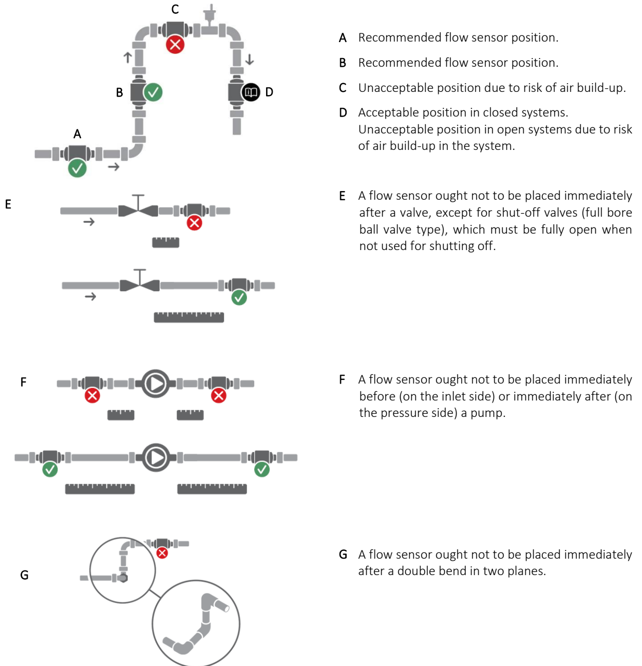
Figure 15. General installation recommendations for flow sensors.
